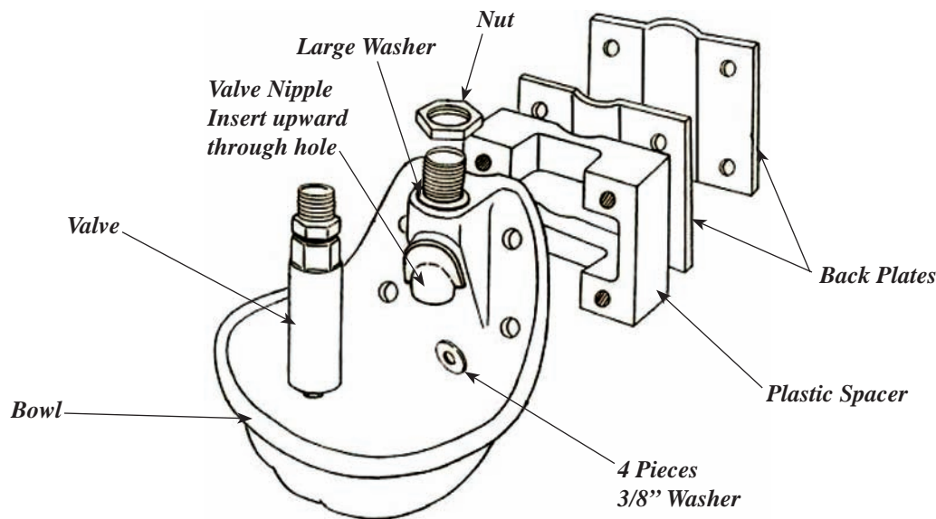
Mounting Arrangement with water supply from below (using plastic spacer)
