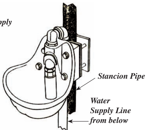
Mounting Arrangement with water supply from below (using plastic spacer)
